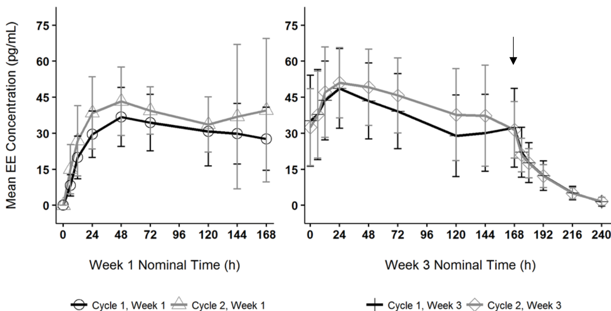
Figure 4. Mean Serum Ethinyl Estradiol Concentrations in Healthy Female Volunteers Following Two Consecutive Cycles of TWIRLA Wear on the Buttock (Vertical arrow indicates time of TWIRLA removal)
